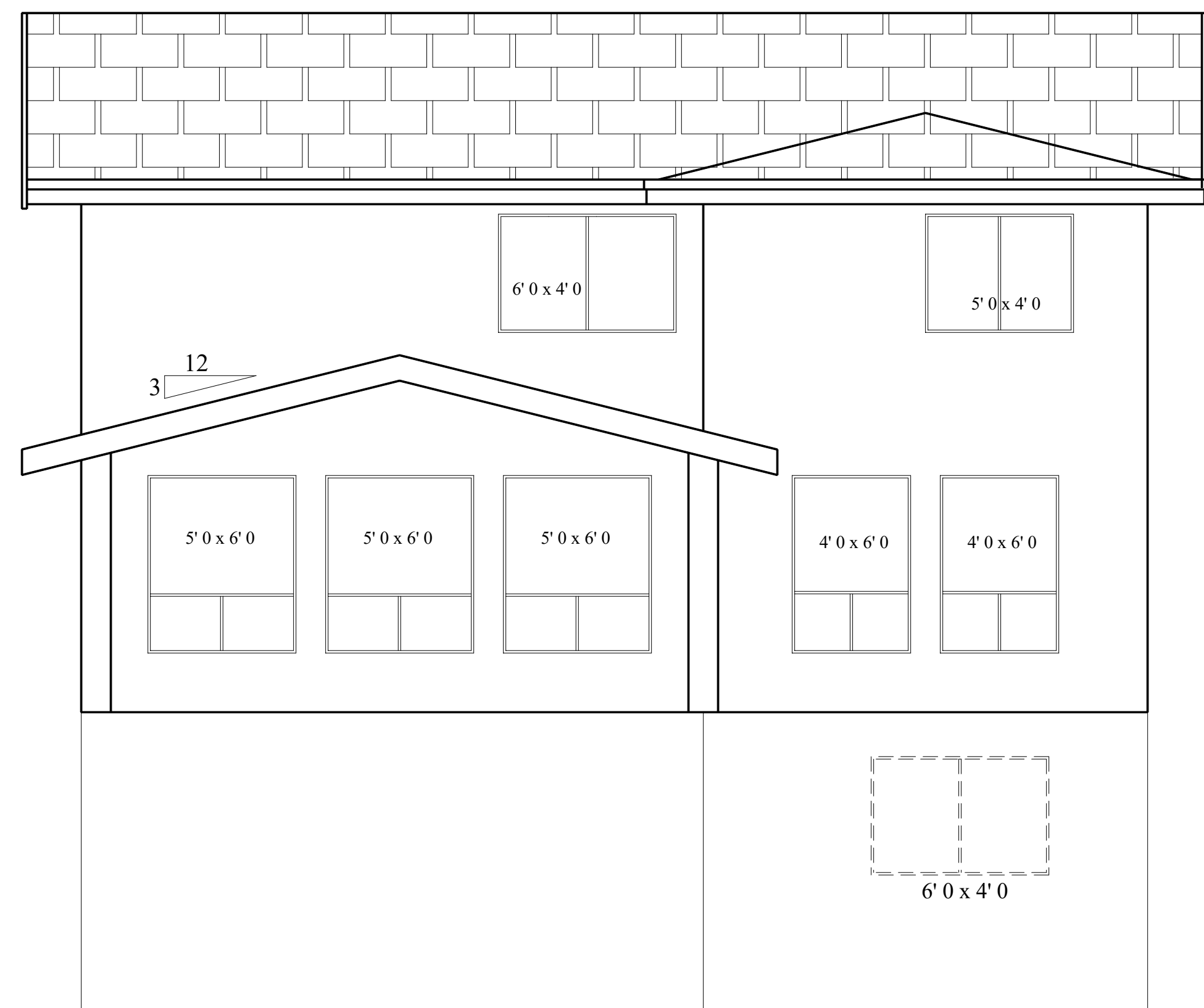
REAR ELEVATION
