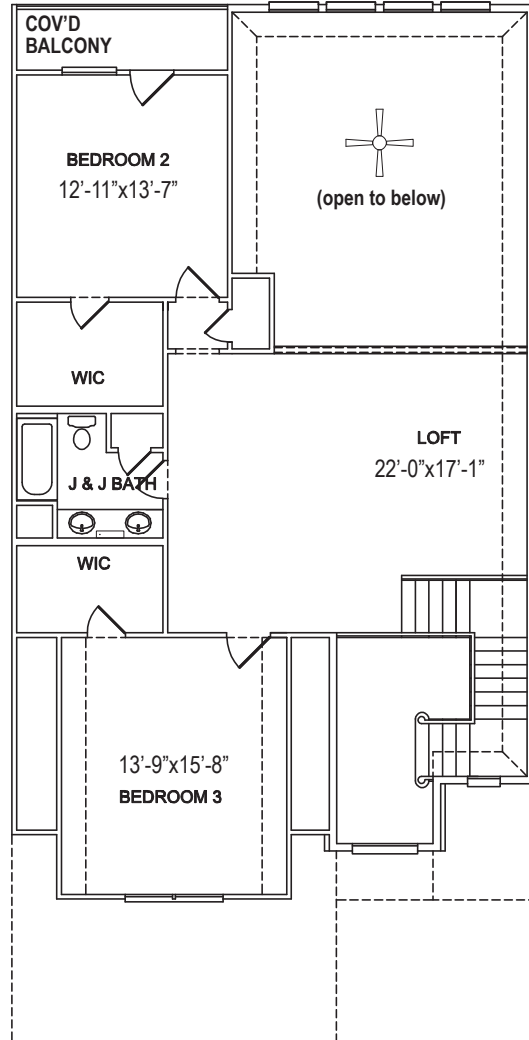
SECOND FLOOR
